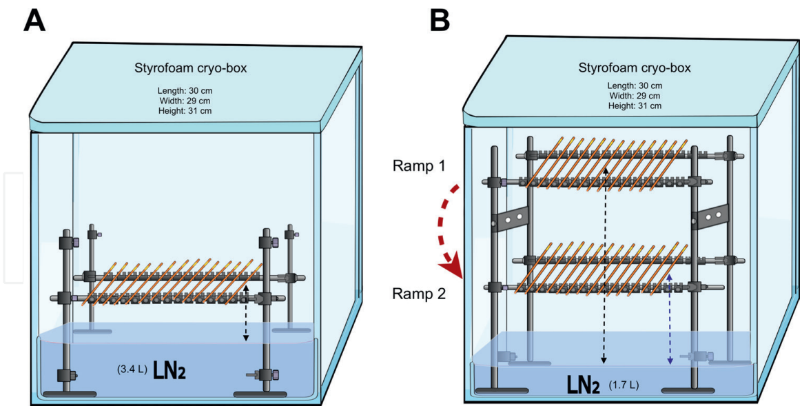
Figure 5. Styrofoam cryo-boxes are used for cryopreserving domestic spermatozoa by conventional slow freezing. The conventional cryo-box has one freezing ramp located 4 cm from the LN 2 surface. The modified cryo-box has two freezing ramps located at either 7 and 17 cm or 10 and 24 cm from the LN 2 surface.
