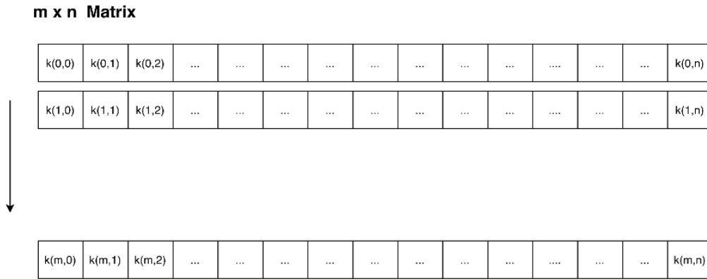
Figure 3: m \times n matrix of initial candidate solutions.
