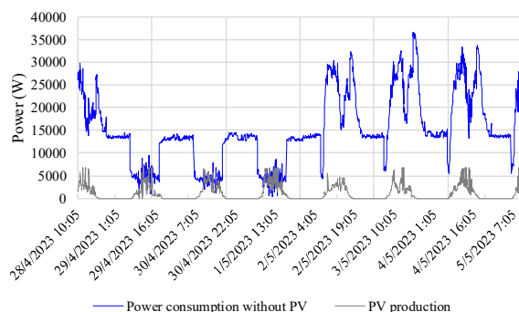
Figure 4: Real power consumption profile vs PV production.
