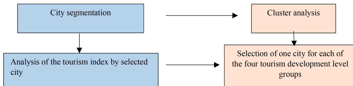
Fig. 1. Methodological diagram.
