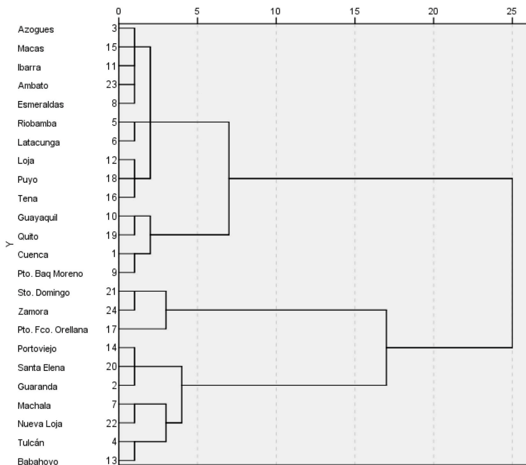
Fig. 2. Dendrogram that uses Ward's method. Combination of re-scaled distance clusters. Source: Authors' own.
