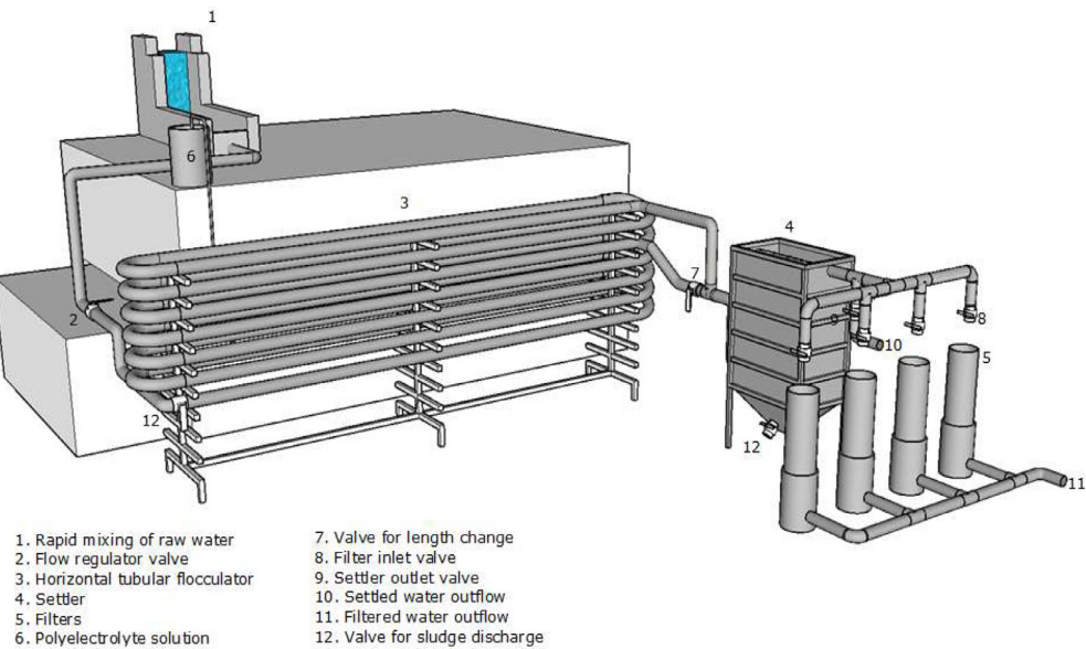
Fig. 1. Pilot system for the treatment of drinking water, this system includes a horizontal flow tubular flocculator.
