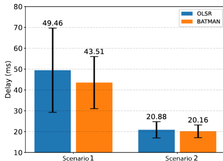
Figure 9. Average delay
