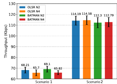
Figure 11. Average throughput
