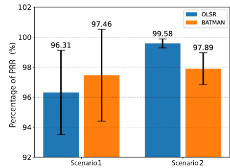
Figure 10. Average PRR
