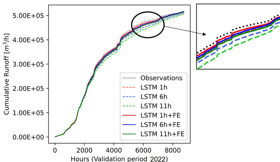
FIGURE 12 Comparison of cumulative runoff values for referential and specialized models.
