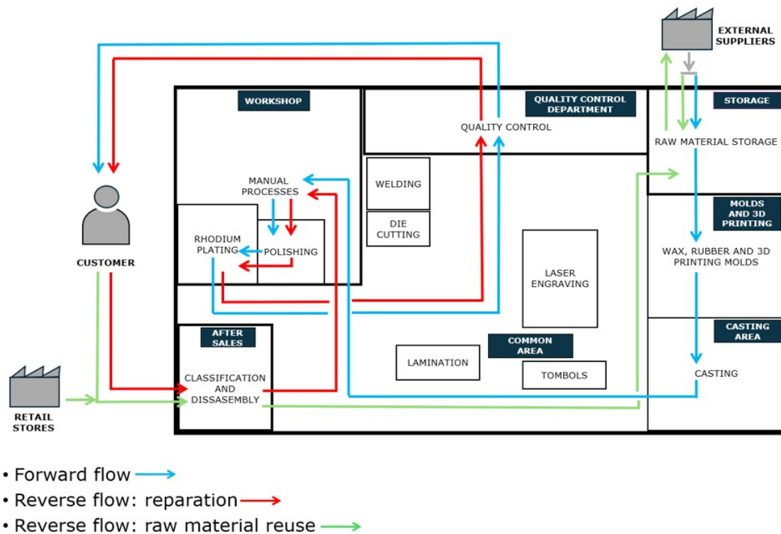
Figure 1. Scheme and flows of the facility layout of the jewelry factory in the application case
