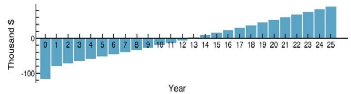
Fig.5. Annual investment recovery, considering not power retail price increase.
