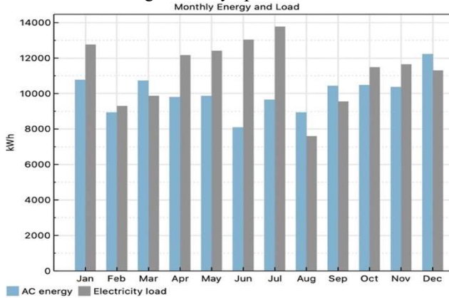
Fig. 4. Monthly power consumption recorded in the year 2019 versus PV potential
