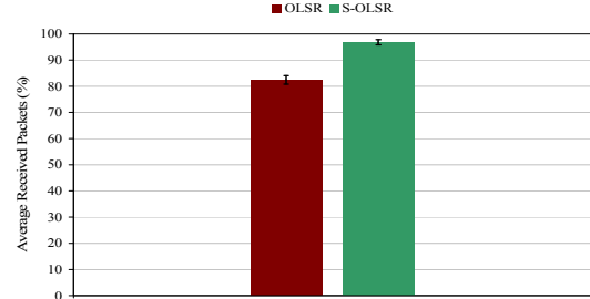
Figure 12: Comparison of average packet reception rate: Standard OLSR and S-OLSR.
