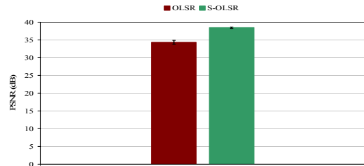
Figure 13: Comparison of average PSNR: Standard OLSR and S-OLSR.
