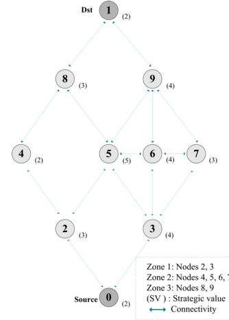
Figure 3: Scenario designed for the evaluation of S-OLSR.
