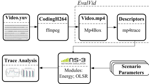
Figure 2: Evaluation methodology for the proposal in the simulation environment.
