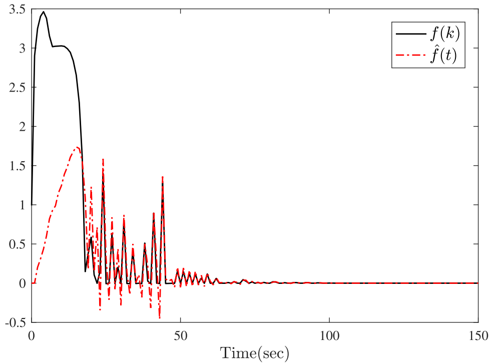
FIGURE 3. The attack signal and its estimated signal.
