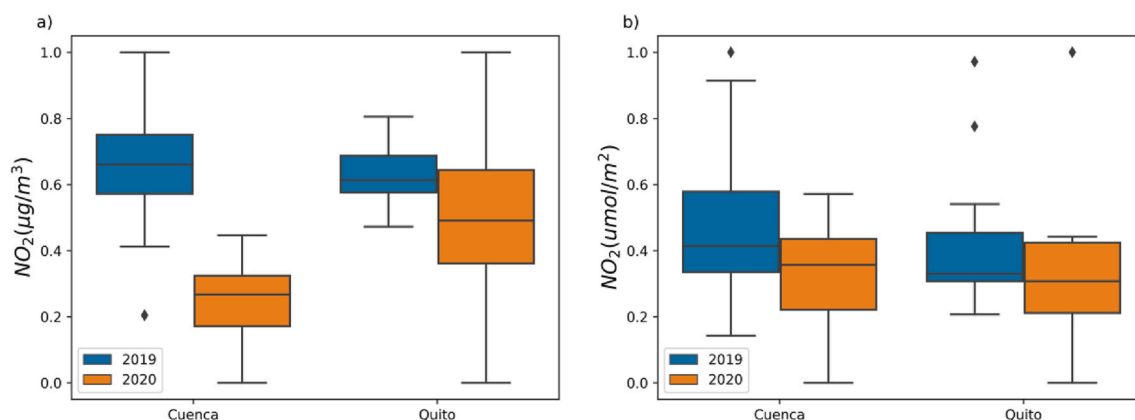
Fig. 4. Box plots of \text{NO}_2 concentrations recorded by a) Ground-based stations and b) Sentinel-5P during the years 2019 and 2020. The box represents the interquartile range (IQR), which spans from the first quartile (Q1) to the third quartile (Q3) and contains the middle 50% of the data. The horizontal line inside the box represents the median of the data set. The whiskers on the box extend to the most extreme values within a range calculated based on IQR; points outside these limits are considered outliers.
