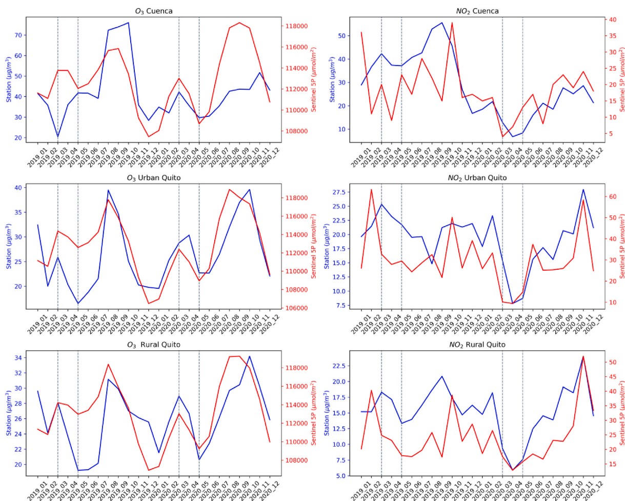
Fig. 2. Behavior of ground-based vs Sentinel-5P data for O 3 and NO 2 in the cities of Quito and Cuenca during 2019 and 2020.
