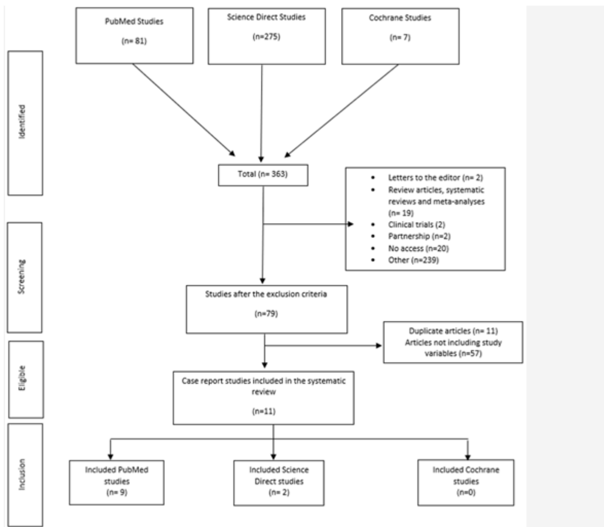
Figure 1: Flow chart showing the methodology used in the selection of studies for full analysis.
