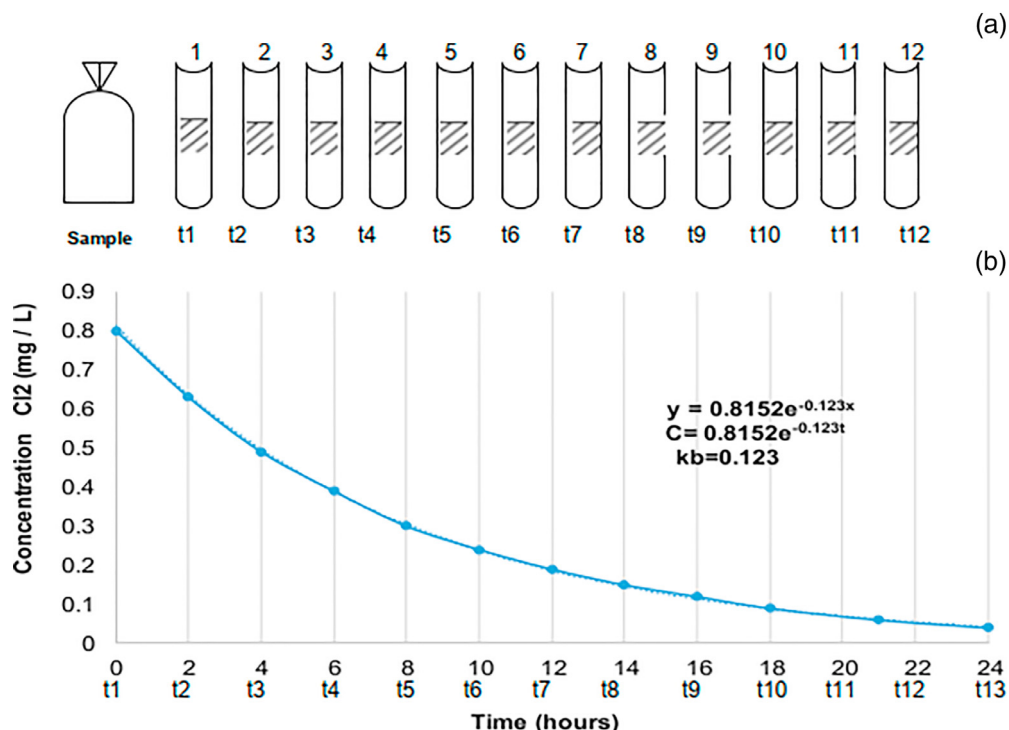
Fig. 2. Laboratory Bulk Decay Coefficient Determination Diagram: (a) Bulk Decay Bottle Tests, (b) First order exponential fit for the equation.
