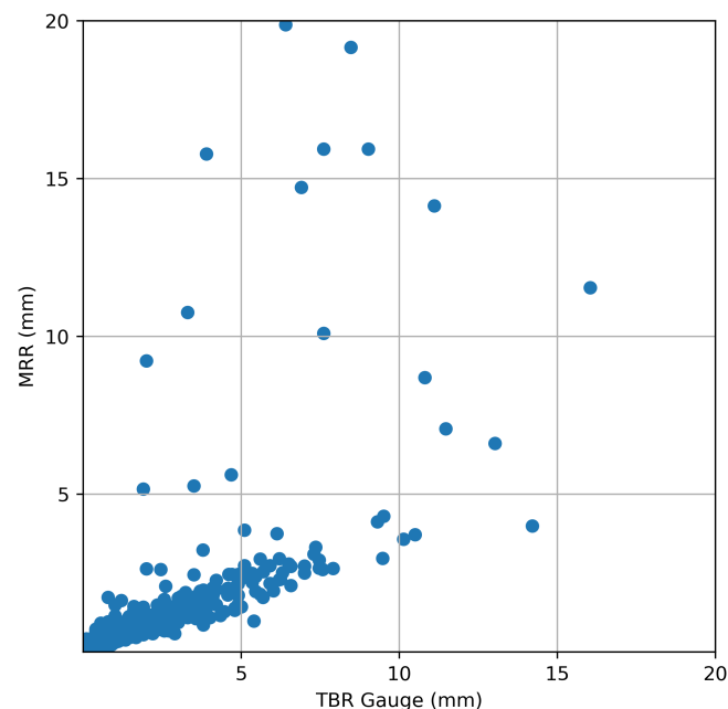
Figure 2. Scatterplot between the hourly precipitation amounts recorded by the MRR and the collocated tipping bucket rain (TBR) gauge in Cuenca.
