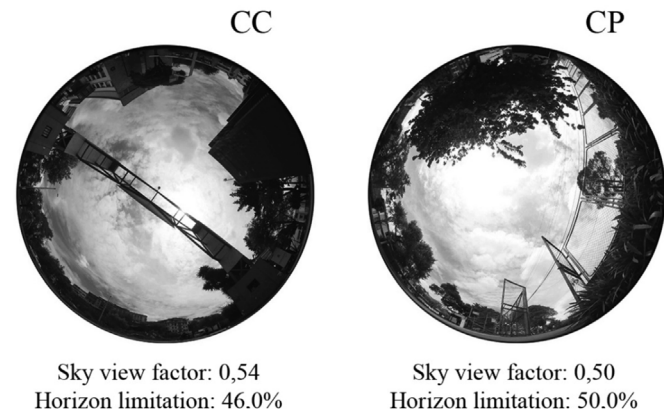
Fig. 1. Fish-eye images and SVF values in the two study sites.
