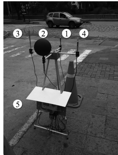
Fig. 3. 1) Temperature probe 2) Globe thermometer probe 3) Hot wire probe 4) Combined probe; temperature and relative humidity 5) Data logger.
