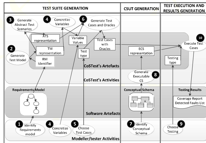
Figure 1. The CoSTest process
