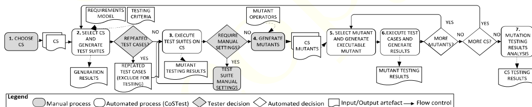
Figure 4. Steps taken in experimental process
