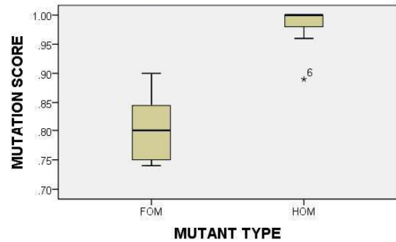
Figure 8. Box-plot of data for Test Suite Adequacy
