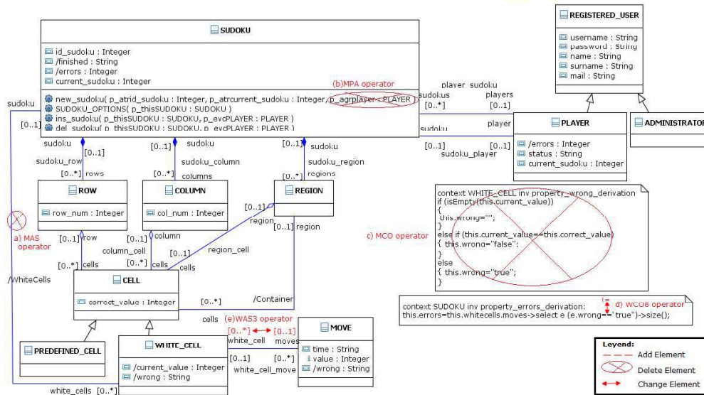
Figure 3. Excerpt of a UML CD-based CS and the application of five mutation operators
