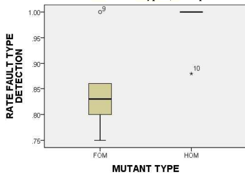
Figure 7. Box-plot for FTDR by Mutant Type
